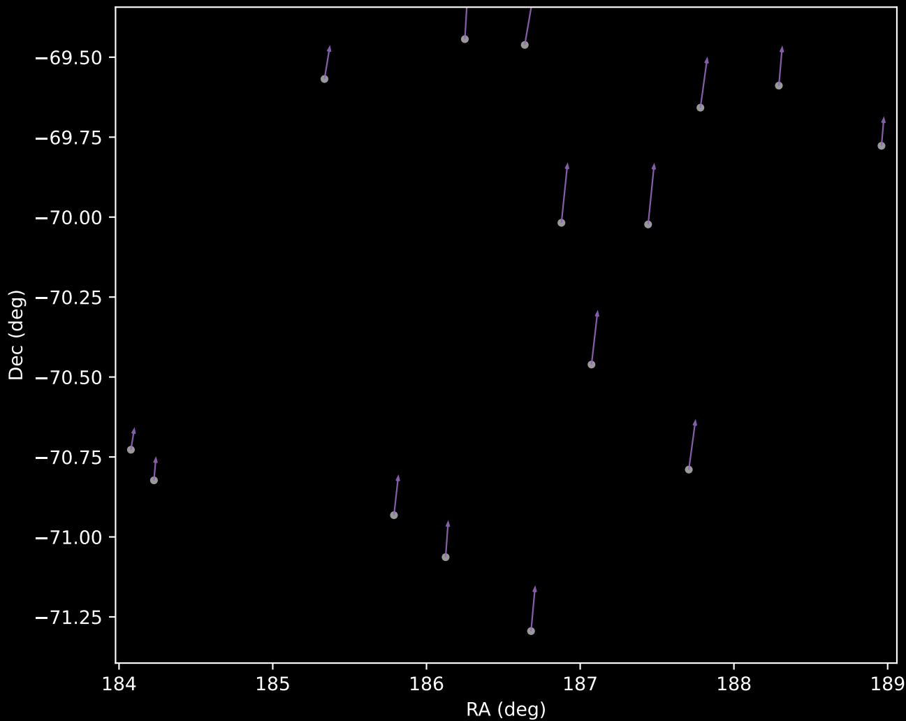
GALAH DR4 Cluster 8 Proper Motion Vectors (n=15)
