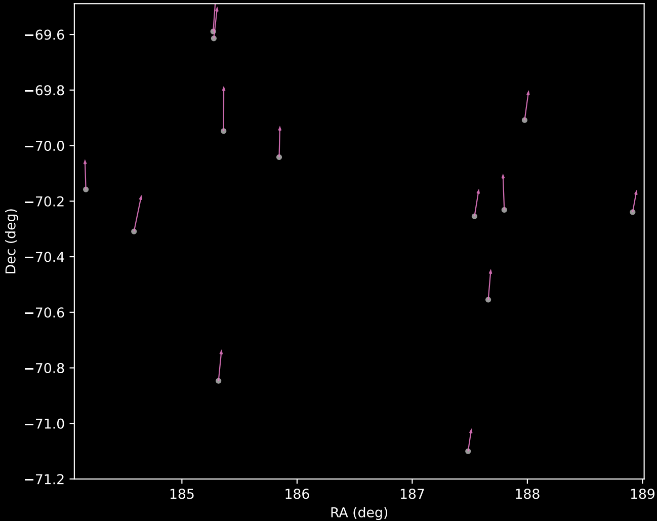
GALAH DR4 Cluster 12 Proper Motion Vectors (n=13)
