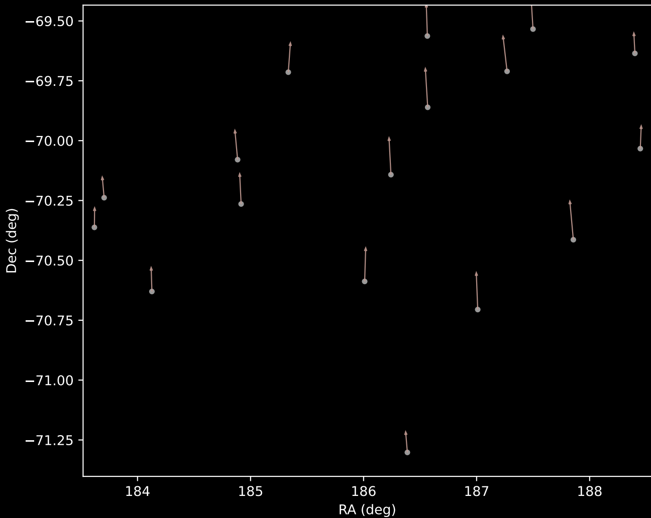
GALAH DR4 Cluster 11 Proper Motion Vectors (n=17)
