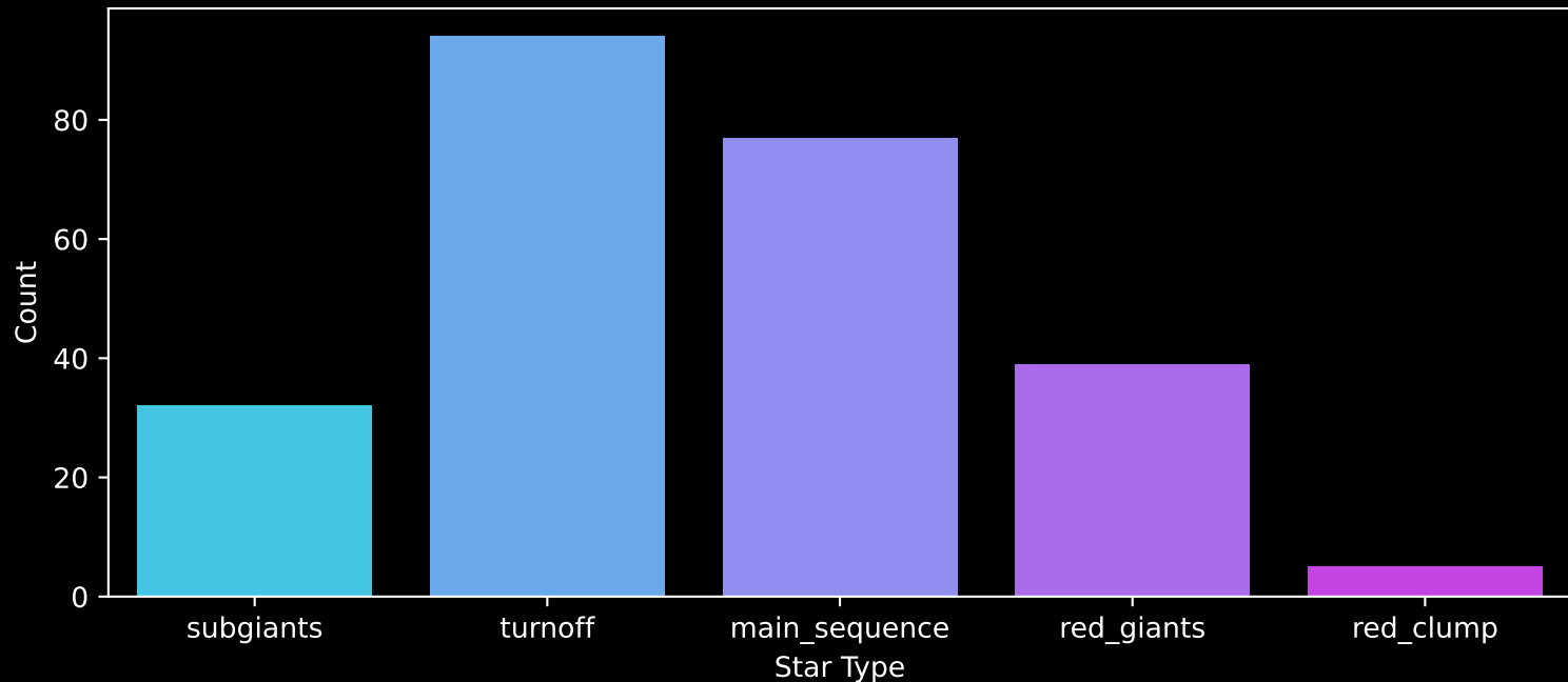
GALAH DR4 Field: [7134] Count plot of Star Type
