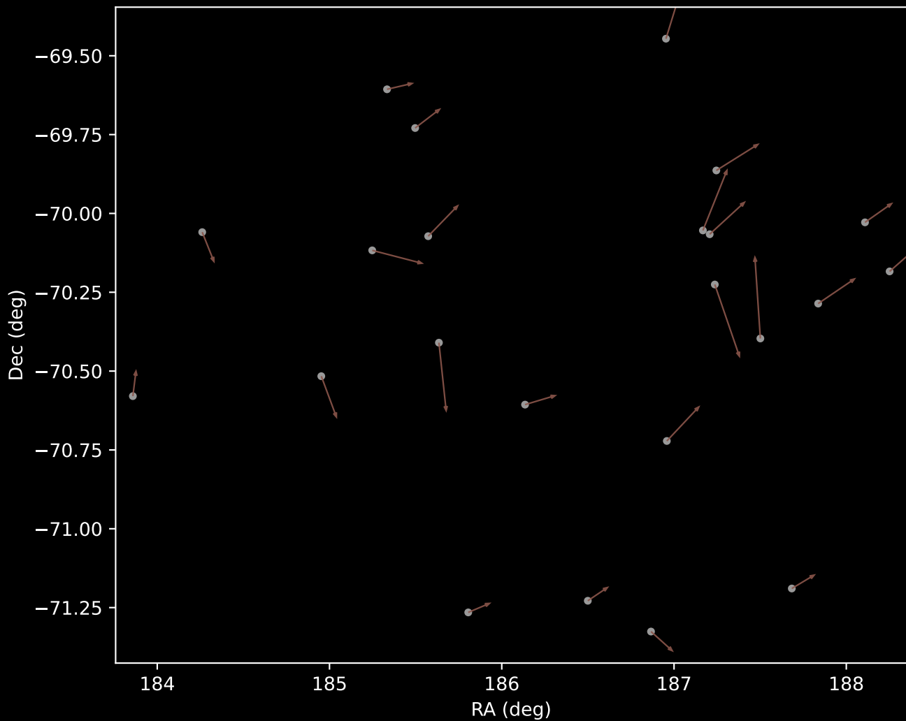
GALAH DR4 Cluster 10 Proper Motion Vectors (n=23)
