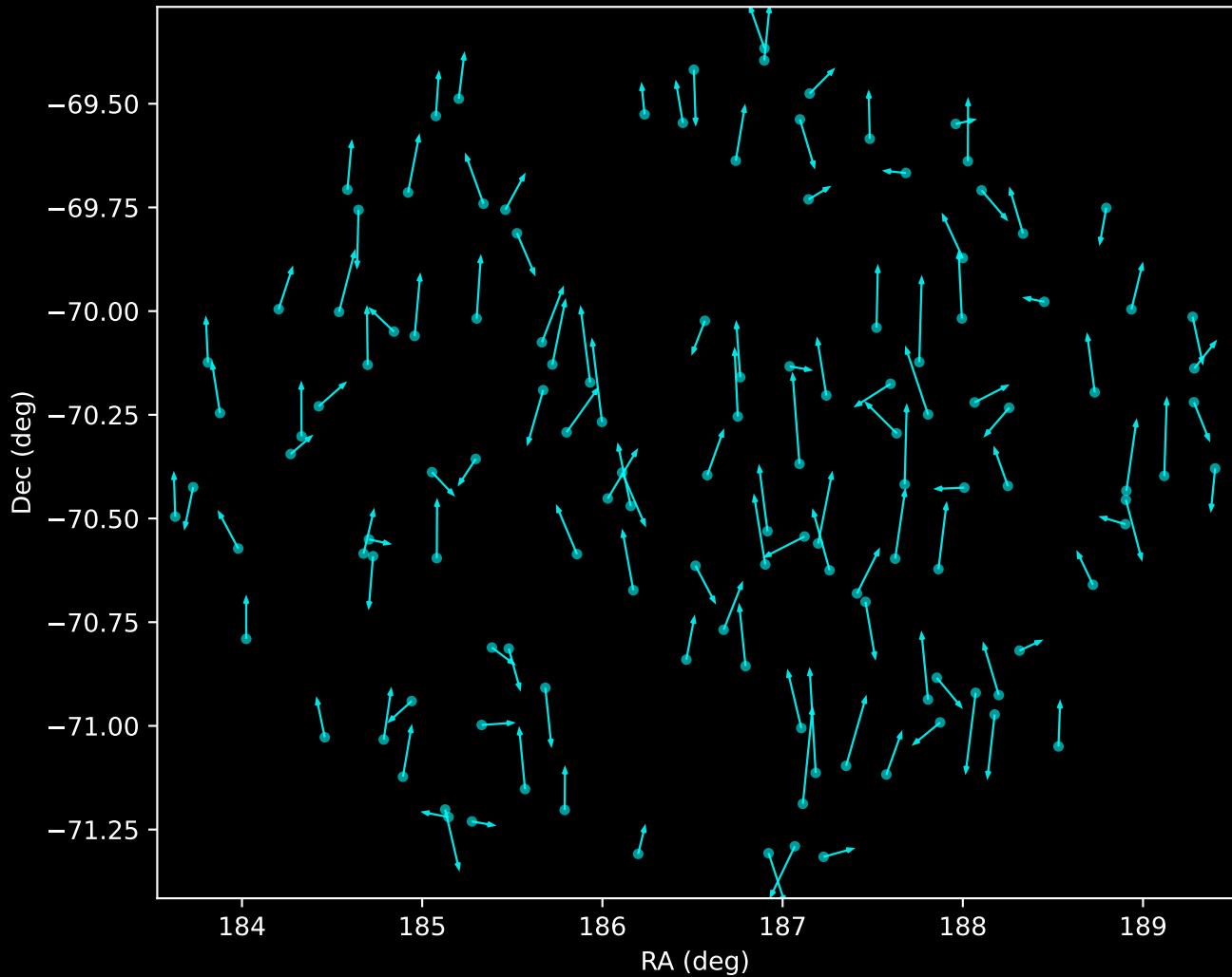
GALAH DR4 Noise Stream Proper Motion Vectors (n=130)
