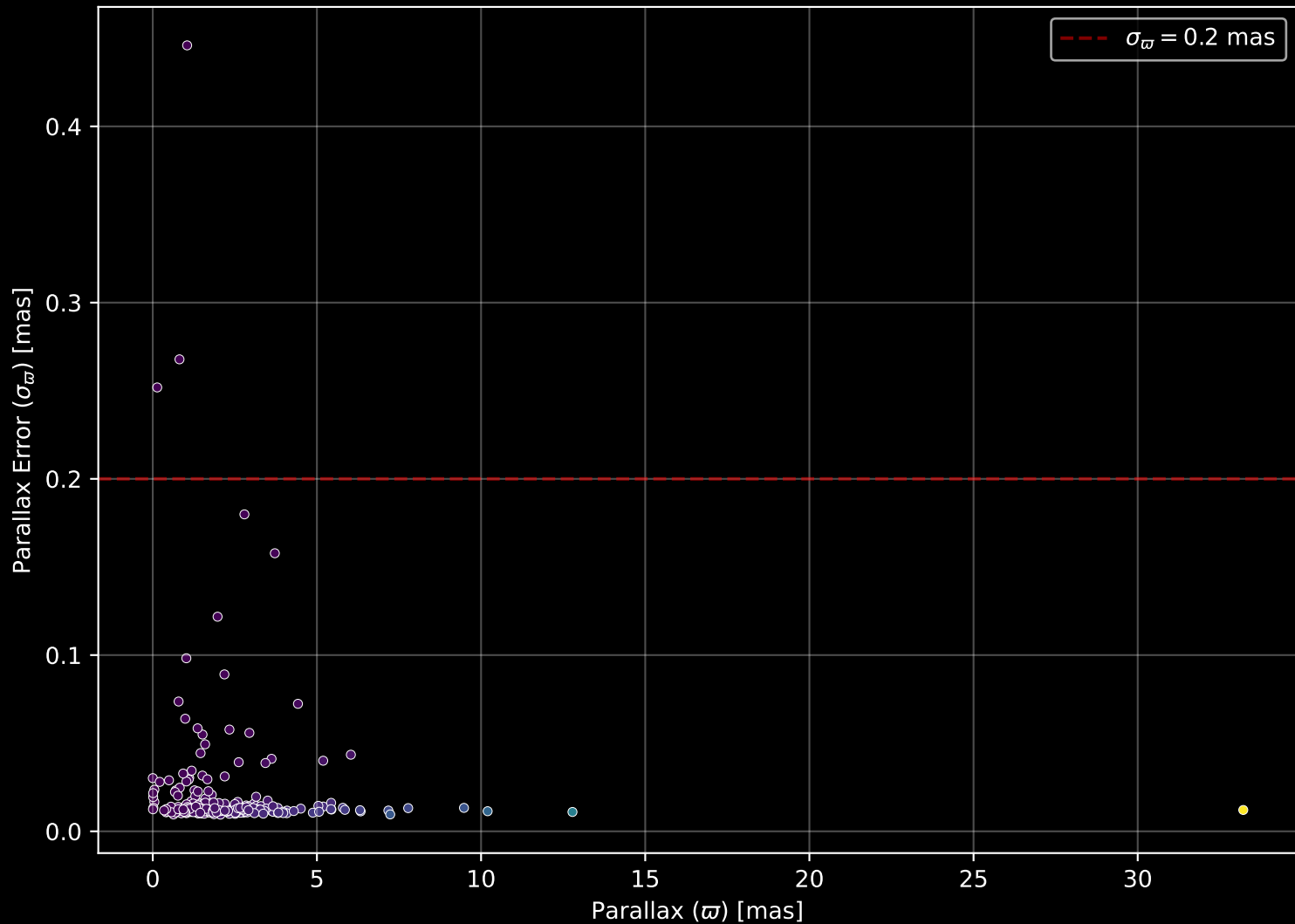
GALAH DR4 Field: [7134] Parallax Quality (n= 247)
