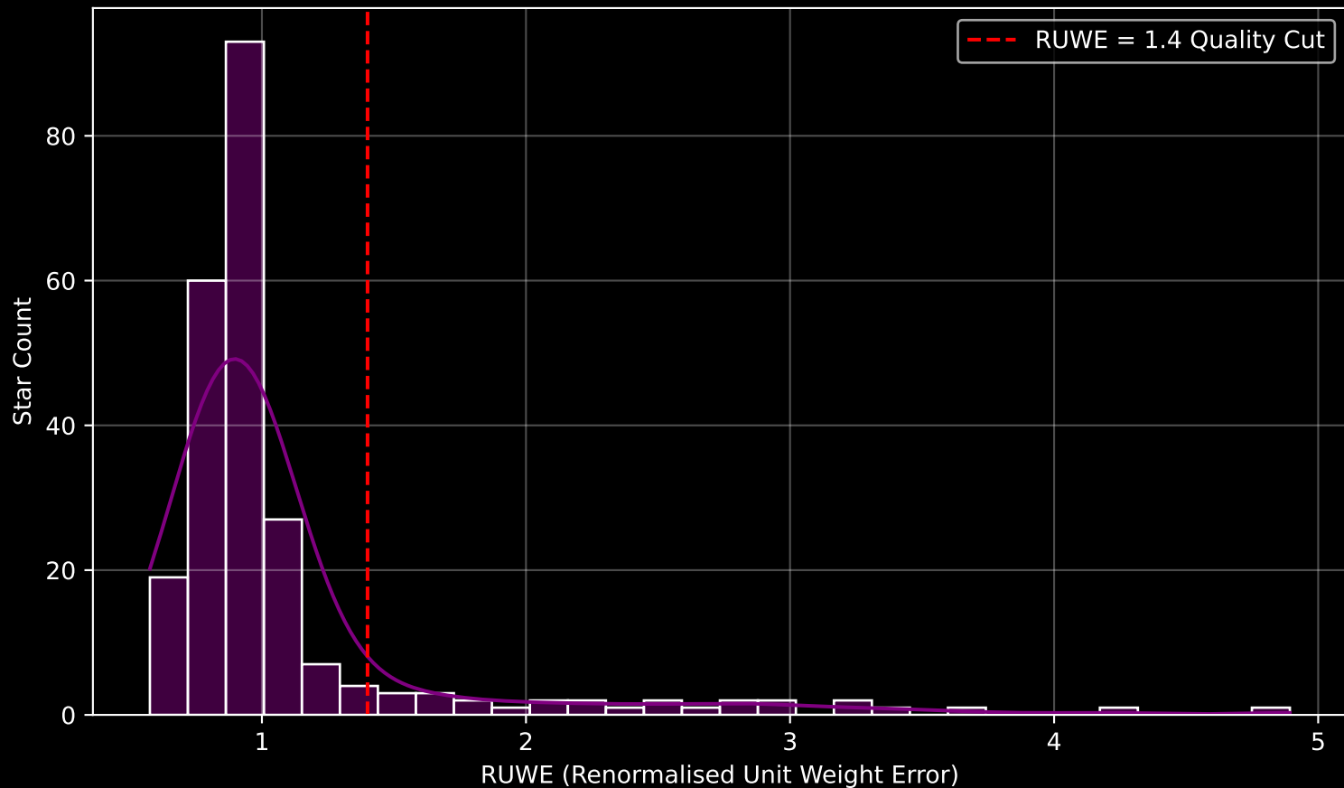
GALAH DR4 Field [7134] RUWE Distribution (n= 237)
