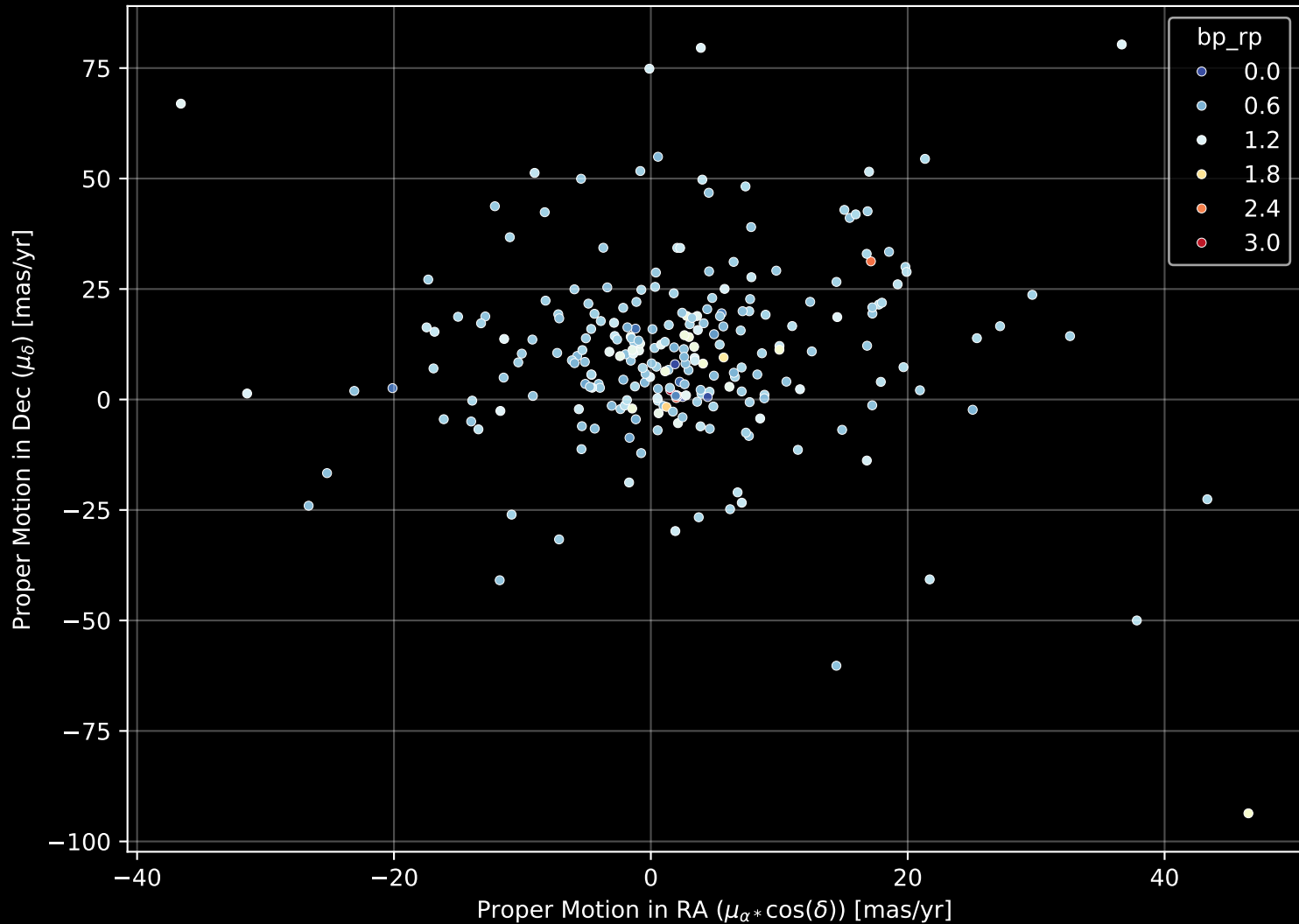
GALAH DR4 Field: [7134] Proper Motion Diagram (n= 247)
